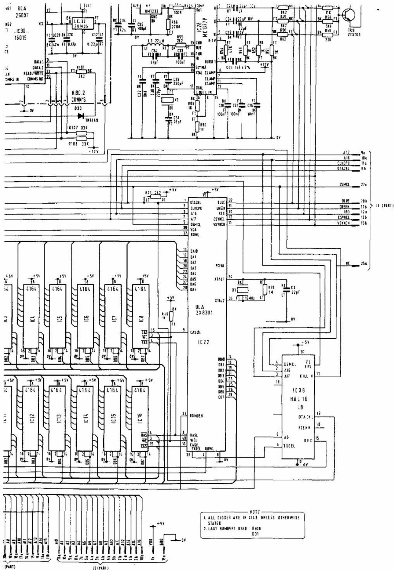
FIGURE 1.5 QL CIRCUIT DIAGRAM (Issue 6) 1.18
