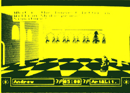
Genus II
